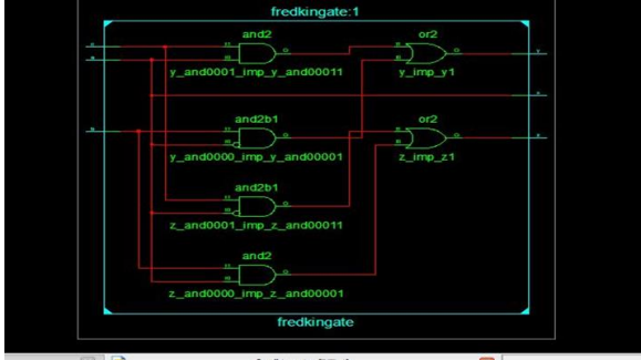
Fig. 5. RTL schematic of URL Gate
