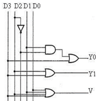
Fig. 1. Existed block diagram of priority encoder
