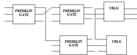
Fig. 2. Proposed block diagram of priority Encoder Using Reversible logic gates
